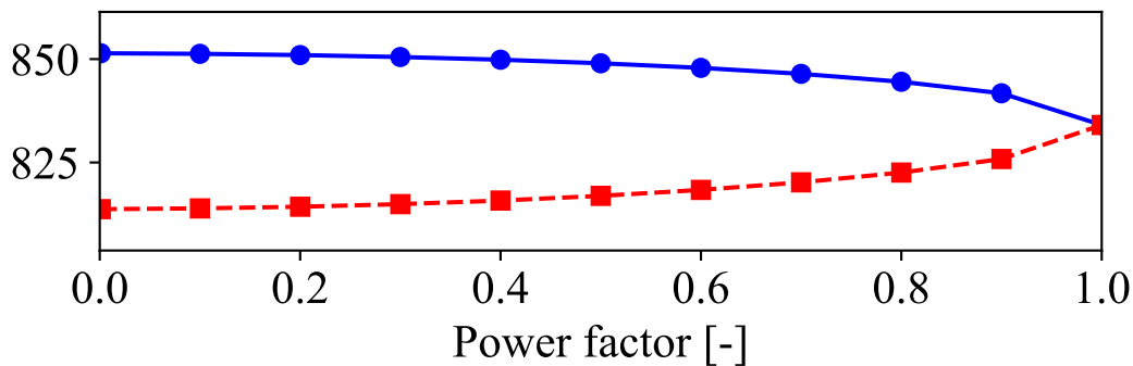
Inverter-side inductor L1
